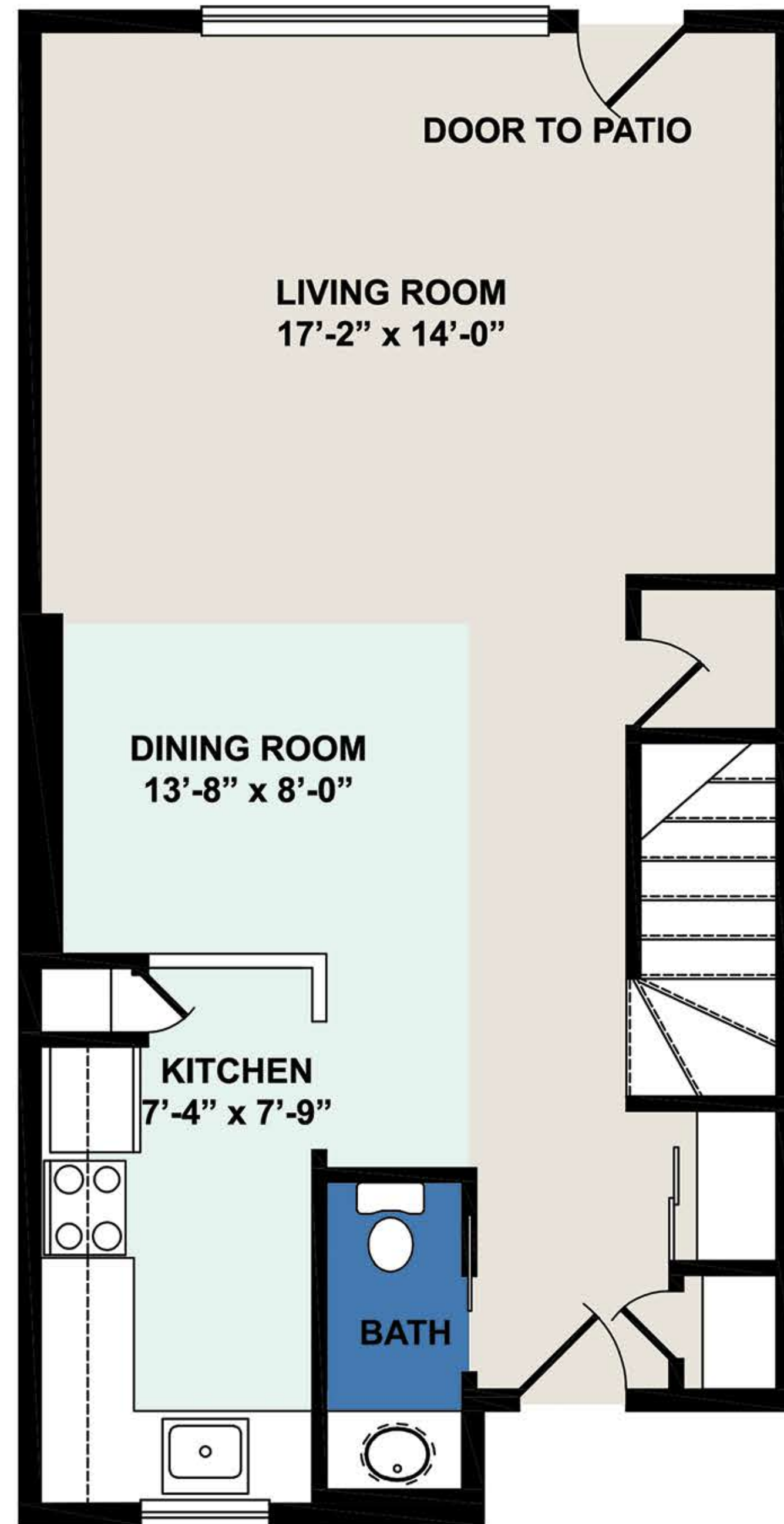
MAIN FLOOR
