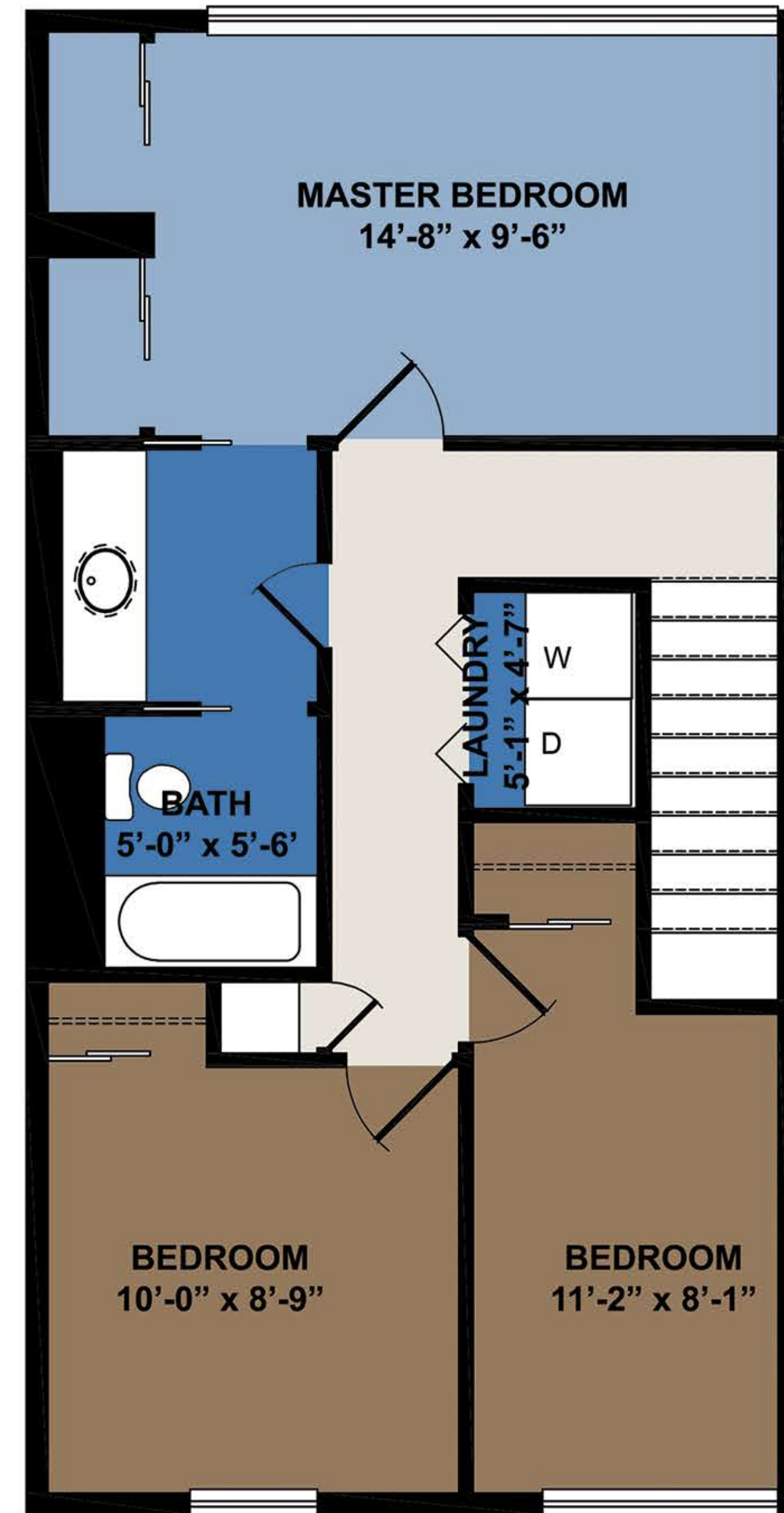
SECOND FLOOR
